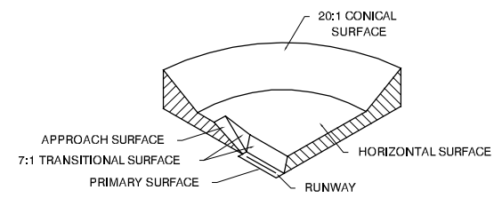
TYPICAL FAR PART 77 SURFACES
